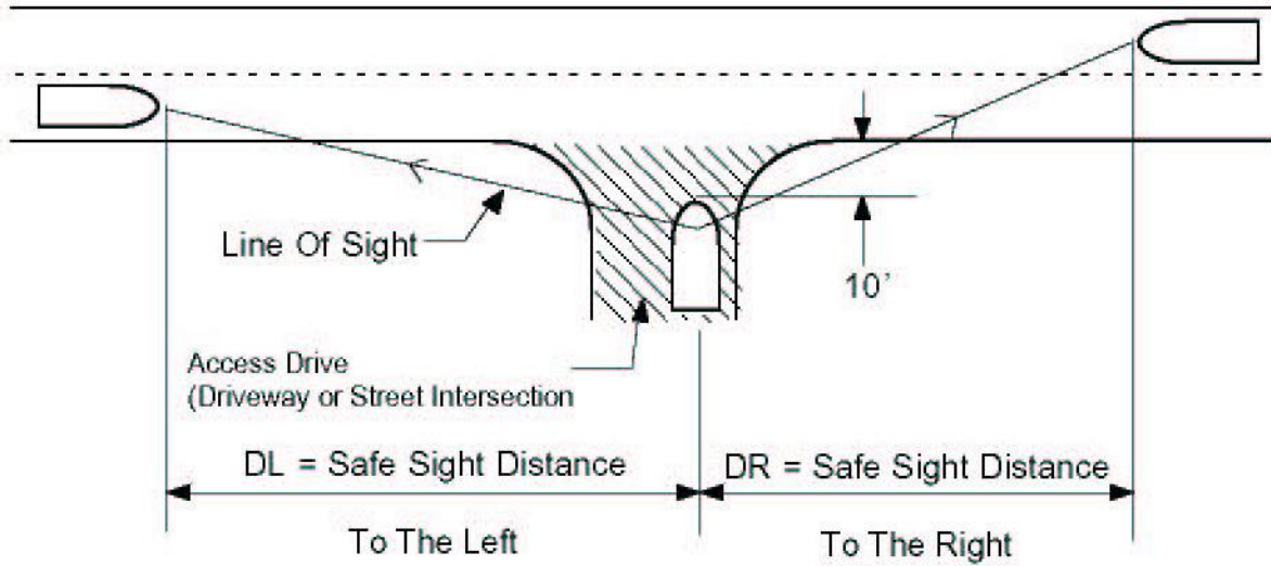
FIGURE 1A SIGHT DISTANCE FOR VEHICLES EXITING FROM ACCESS POINTS refer to Table 1A
