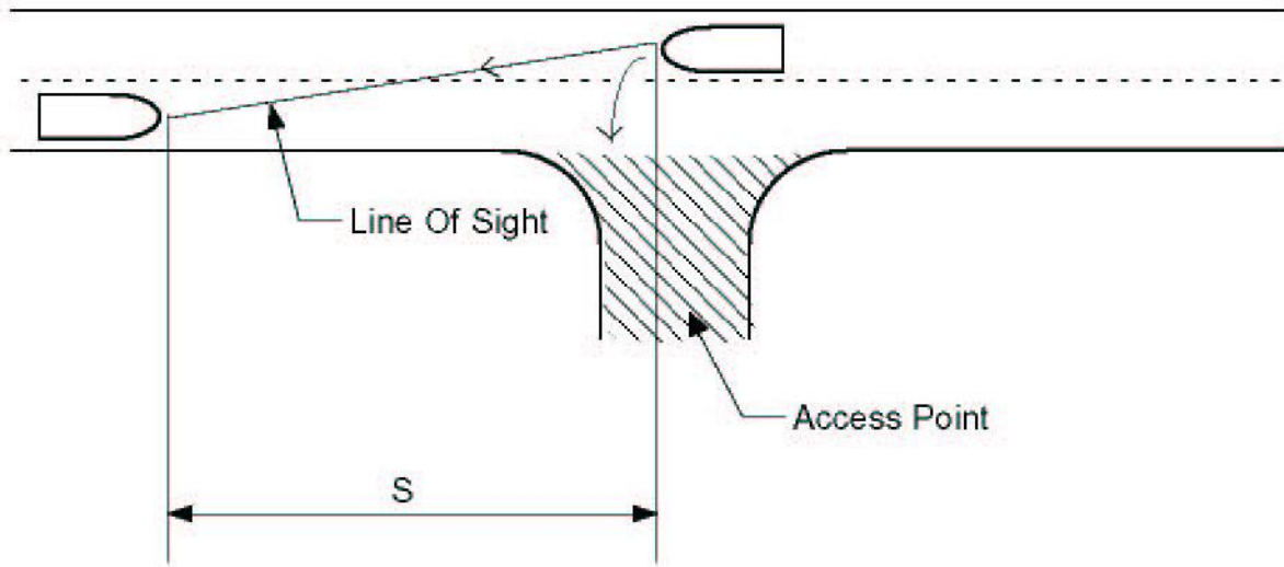
FIGURE 1B LEFT TURN SIGHT DISTANCE FOR VEHICLES ENTERING ACCESS POINTS refer to Table 1B
