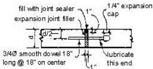
EXPANSION JOINT
