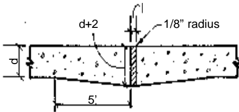
ALTERNATE EXPANSION JOINT
