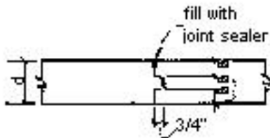
LONGITUDINAL CONSTRUCTION JOINT KEYWAY
