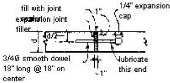
EXPANSION JOINT
