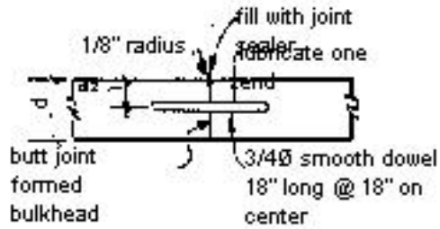
TRANSVERSE CONTRACTION JOINT (PLANNED - COINCIDE WITH CONTRACTION JOINT)
