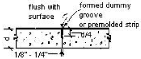
TRANSVERSE CONTRACTION (SAWED OR PREMOLDED STRIP)
