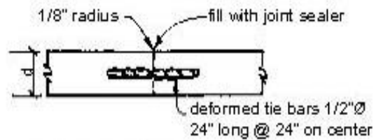
TIED TRANSVERSE CONSTRUCTION JOINT (EMERGENCY - NON COINCIDE WITH CONTRACTION JOINT)
